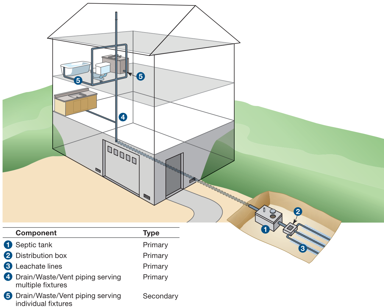
Figure 4-21. DWV system that discharges into an onsite waste disposal (septic) system.
