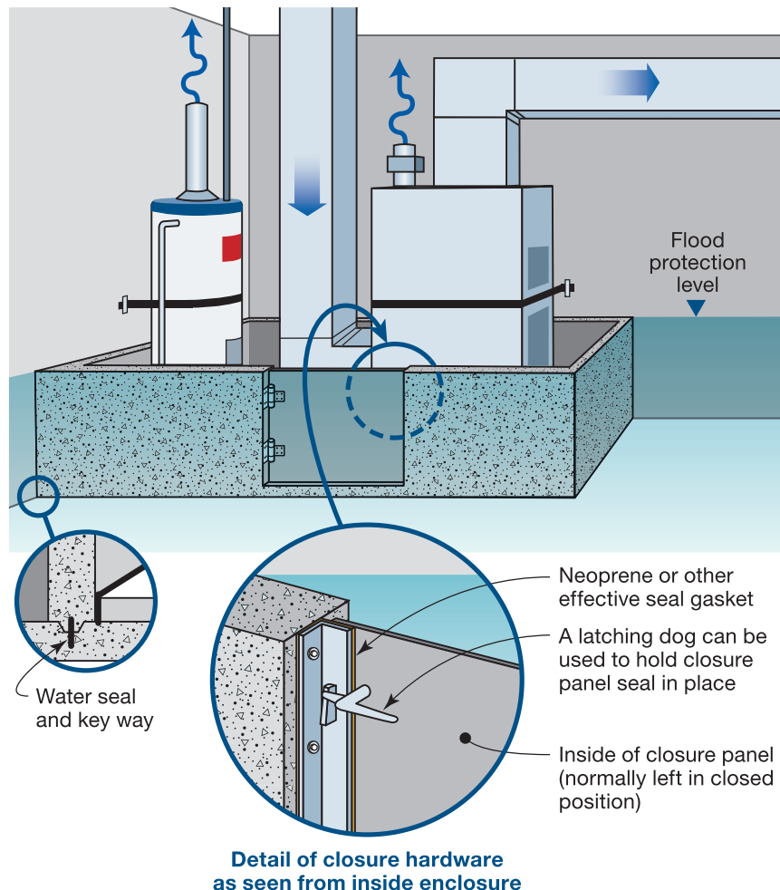
Figure 4-7. Dry floodproofing with a watertight wall and access gate used to protect mechanical and plumbing equipment.
