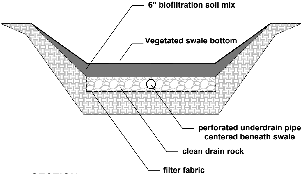
SECTION NTS
