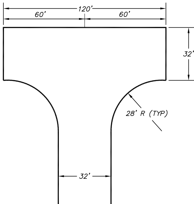
60' HAMMERHEAD
