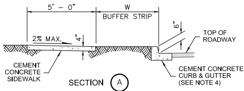
SECTION A
