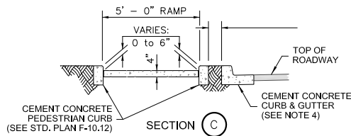
SECTION C
