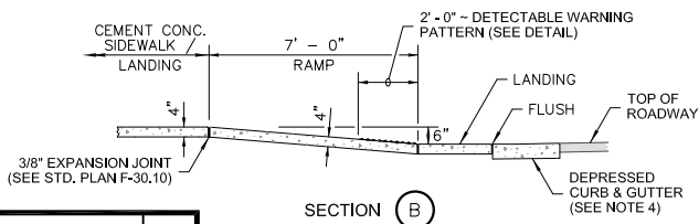
SECTION B
