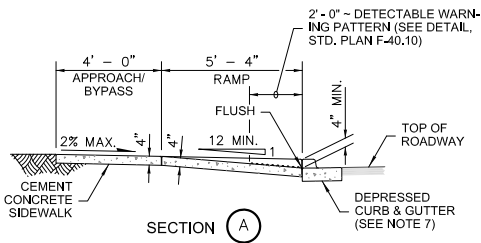
SECTION A
