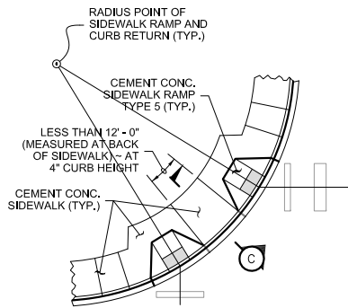
PLAN VIEW LAYOUT 1 SEE NOTE 6
