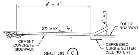
SECTION C
