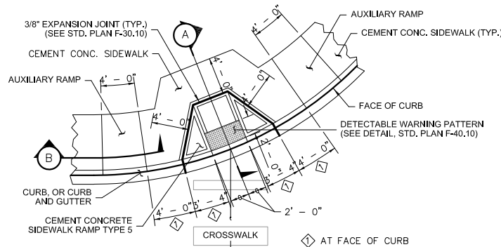
PLAN VIEW SIDEWALK RAMP TYPE 5 FOR LAYOUTS 1, 2, & 3
