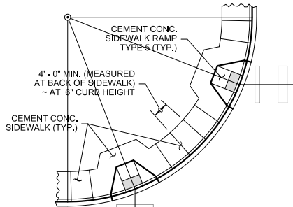
PLAN VIEW LAYOUT 2 SEE NOTE 6
