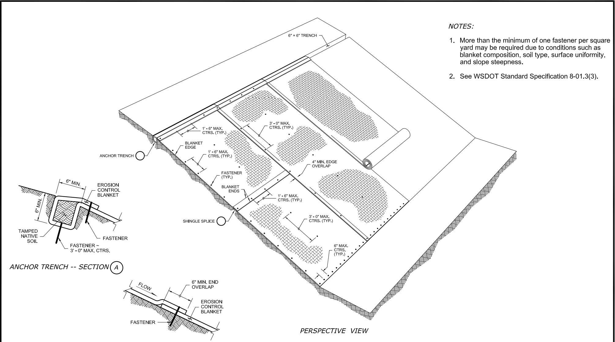
SHINGLE SPLICE -- SECTION (B)
