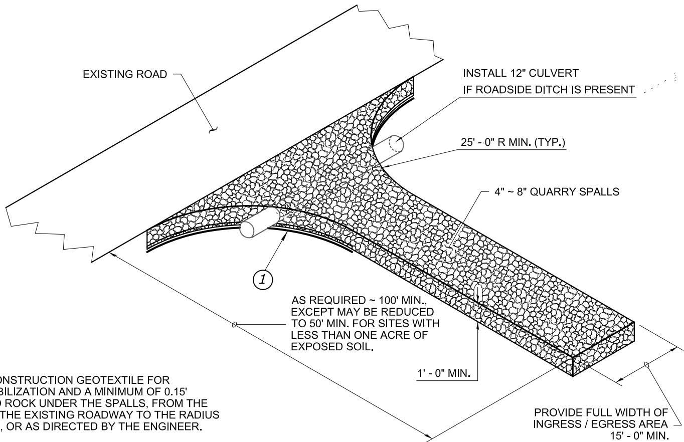
ISOMETRIC VIEW
